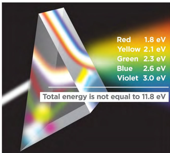
Figure 4. White light entering from the left is spatially separated by a prism into its component colors. The total energy contained in white light is not the sum of the energies of the colors (frequencies) that it contains. White light contains visible energies ranging from 1.65 to 3.26 electronvolts (eV). Summing discrete component energies yields 11.8 eV, an energy level that is characteristic of ultraviolet-C radiation, which is well outside the actual distribution of energies. Plus, frequency and energy are each a continuum that would have to be integrated if they were truly additive.
