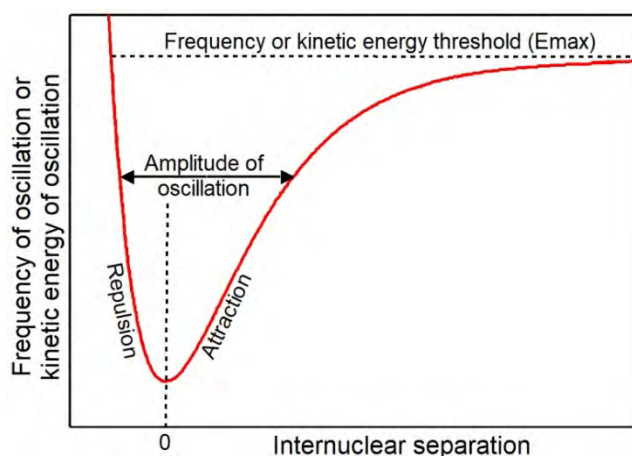
Figure 3. Each bond holding matter together oscillates between electrostatic forces of repulsion on the left and electrostatic forces of attraction on the right. Amplitude of oscillation increases as thermal energy increases. The bond comes apart when thermal energy equals E_{max} . This relationship is known as the Morse potential energy function.
