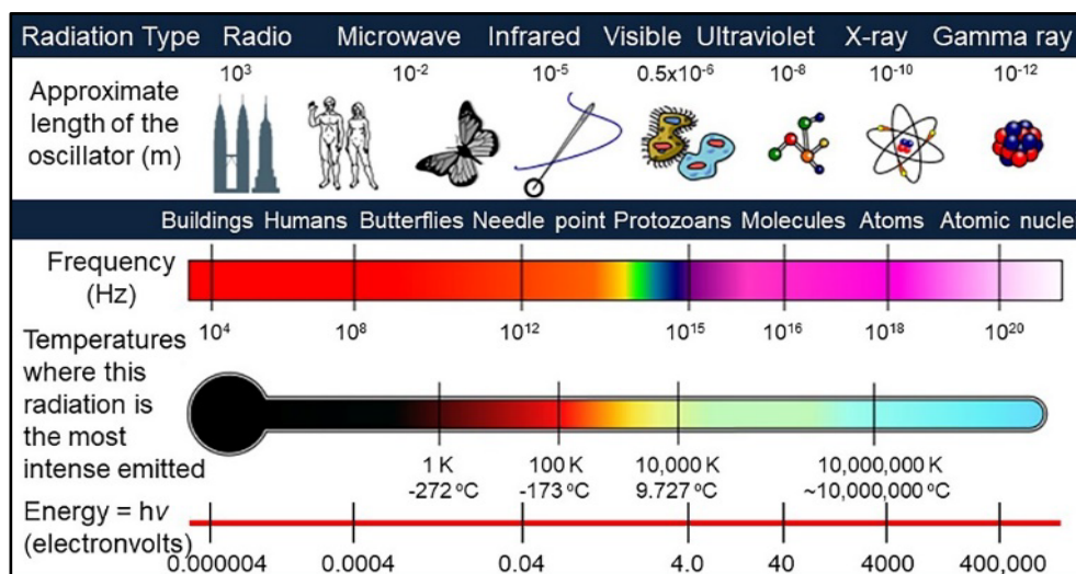
Figure 2. The electromagnetic spectrum extends from radio frequencies of cycles per second to gamma rays with frequencies greater than 300 Exahertz ( 3 \times 10^{20} ). Oscillators with a shorter length emit higher frequency and higher energy radiation associated with higher temperatures.
