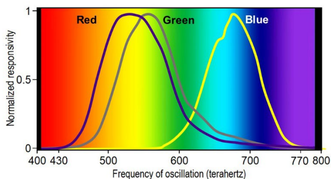
Figure 5. Three different types of cones in your eyes respond in slightly different ways to Red, Green, and Blue light as shown by the solid lines.
