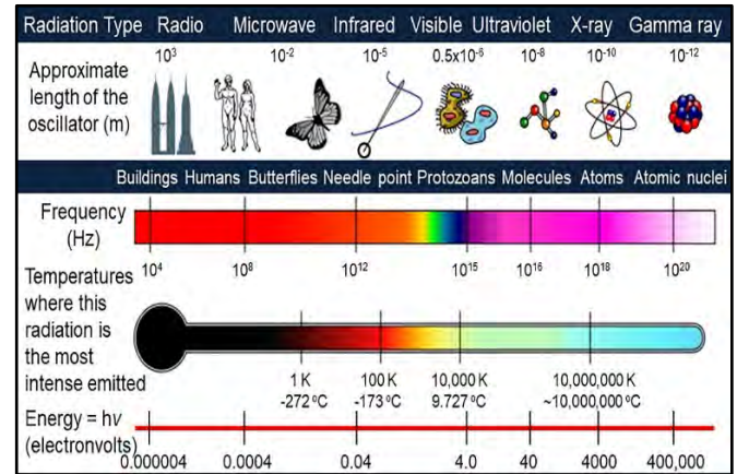
Figure 2. The electromagnetic spectrum extends from radio frequencies of cycles per second to gamma rays with frequencies greater than 300 Exahertz ( 3 \times 10^{20} ). Oscillators with a shorter length emit higher frequency and higher energy radiation associated with higher temperatures.
