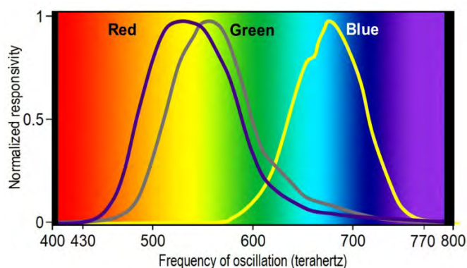
Figure 5. Three different types of cones in your eyes respond in slightly different ways to Red, Green, and Blue light as shown by the solid lines.
