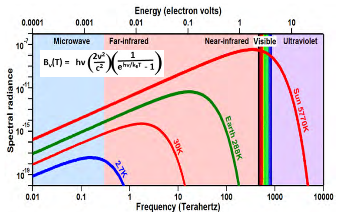
Figure 1. Planck’s law shows that radiation from a warmer body has higher spectral radiance (spectral amplitudes of oscillation) at all frequencies than does radiation from a cooler body and exhibits its greatest amplitude at a higher frequency. Each solid line shows the spectral radiance radiated from a body at thermal equilibrium for the temperature shown. The equation for Planck’s law is shown in the upper left where B_\nu is the spectral radiance written in terms of Planck’s constant ( h ), frequency ( \nu ), velocity of light ( c ), the Boltzmann constant ( k_B ), and absolute temperature ( T ).
